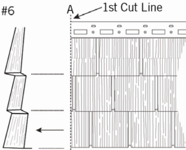
Slide cut-to-fit panel next to corner
