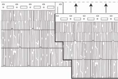
Slide upward making sure to engage the two locking clips and the bottom locking rail.
